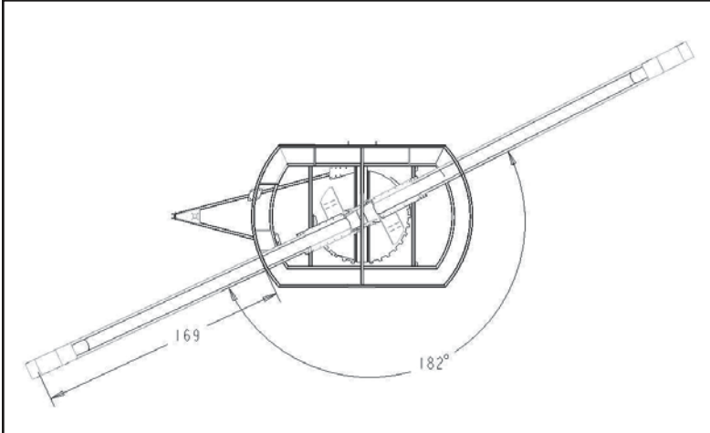
180 degree conveyor swivel with both side and rear unloading positions
